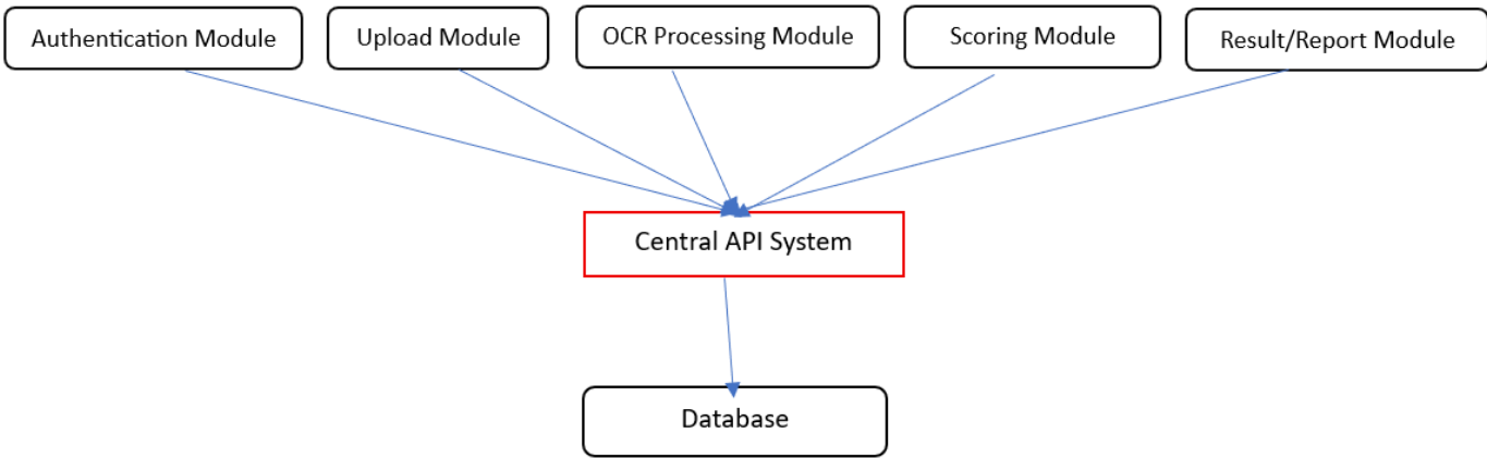
Fig 4.2 Module-Level Architecture
